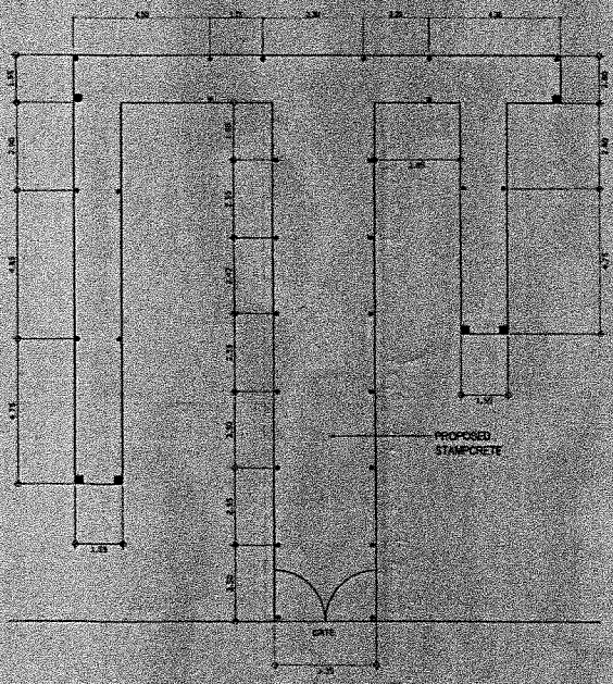
COVERED WALKWAY FLOOR PLAN SCALE: 1:50
