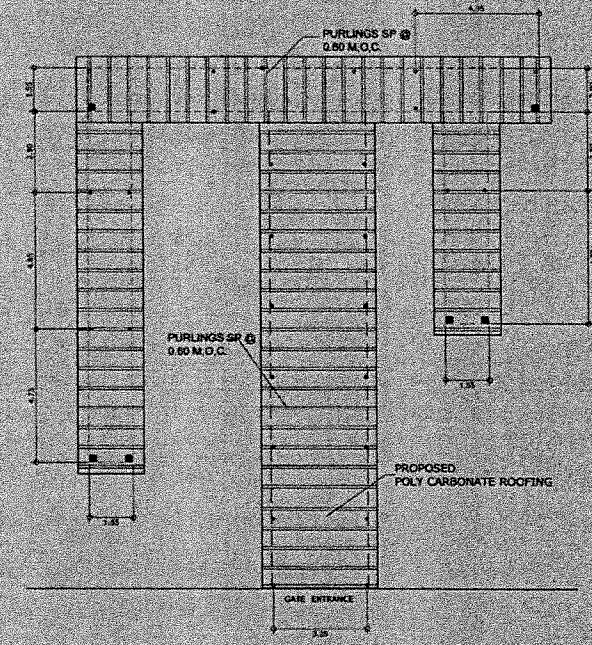
ROOF FRAMING PLAN SCALE: 1:50
