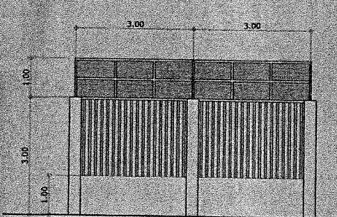
FRONT FENCE ELEVATION SCALE 1/50
